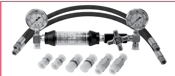
1687102SM Flow Meter Kit For testing and troubleshooting hydraulic systems.
